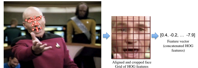
Figure 5: Every face that is uploaded to the game goes through this pipeline. First, a face detector finds locations of landmarks on the face, such as eyes, eyebrows, nose, and mouth. Using those landmark locations, we align the face to a common reference frame and crop the image to just the face region. Then we compute a grid of Histogram of Gradient (HOG) features and concatenate them together to get our final feature vector that we use for classification.
