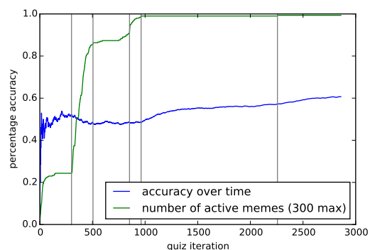
Figure 7: Over almost 3,000 quiz iterations, the game's accuracy (shown in blue) in choosing the correct expression out of three climbs from 33% (random) to above 60%. With more quiz rounds, this number would likely continue to increase. The green line shows how many meme expressions are active in the game, with the vertical bars indicating when more memes were added. Adding new memes, which the system knows nothing about, temporarily hurts performance until the game collects enough examples to learn those memes.
