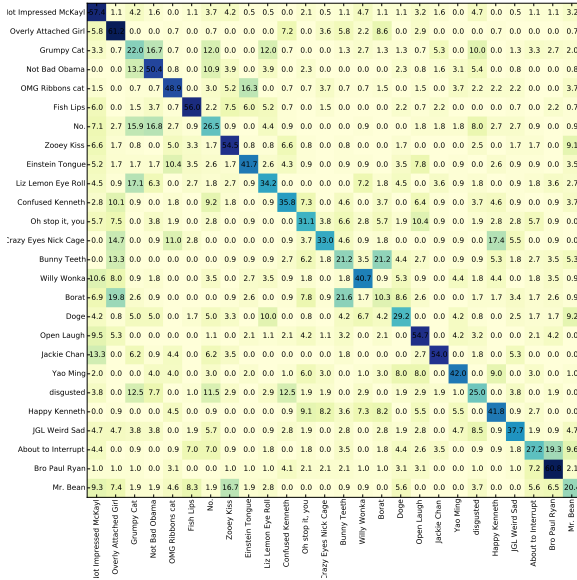
Figure 8: We trained and tested (using cross-validation) a multi-class SVM on the 26 expressions. (Each expression has between 30 and 57 training examples.) This confusion matrix shows which expressions were commonly categorized as other expressions, such as Grumpy Cat with Not Bad Obama. The confusion matrix is not symmetric.
